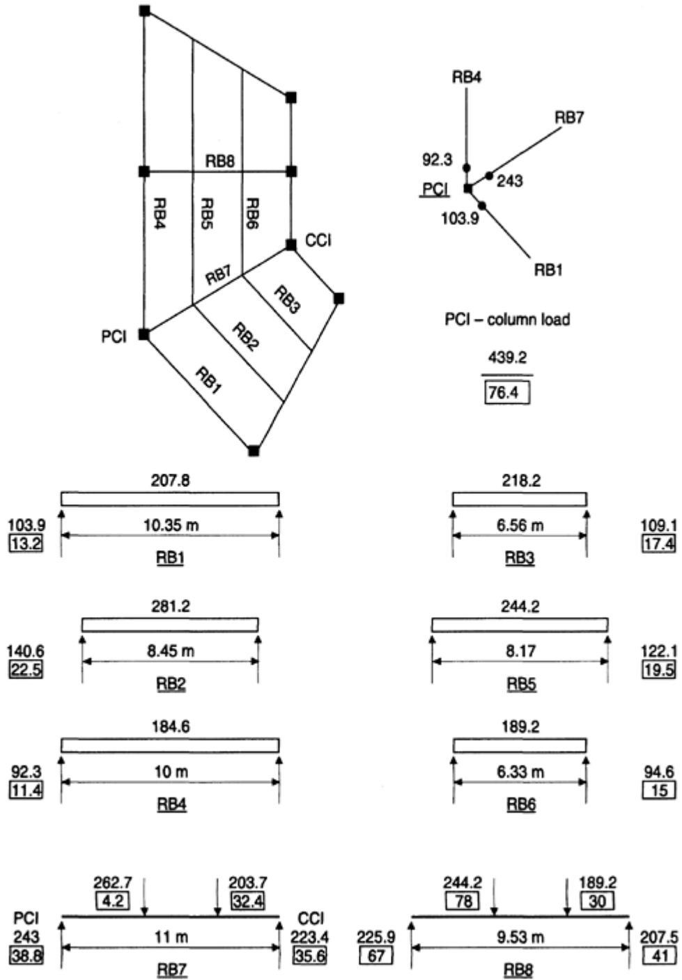
Fig. 7.13 Roof beam loads (kN; unboxed imposed loads shown boxed).
